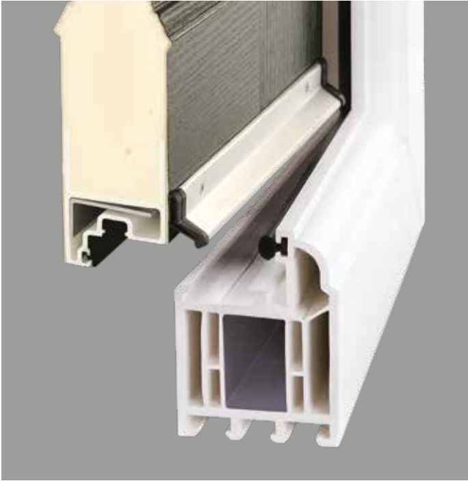
uPVC Full Frame Threshold Distance from bottom of door leaf to bottom of threshold 43mm
